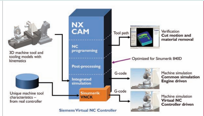
NX controller-driven machine tool simulation
